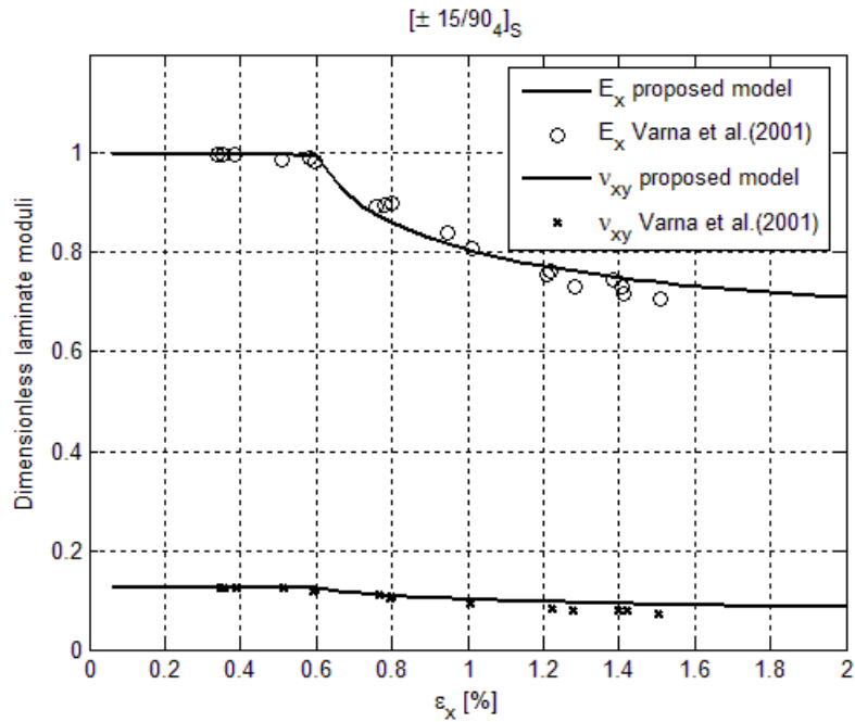
Figure 8. Loss of laminate modulus modulus E_x / \bar{E}_x and v_{xy} as a function of applied strain for a [15/-15/90_4]_S laminate.
