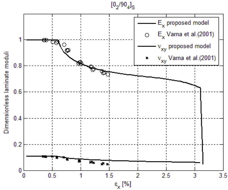
Figure 7. Loss of laminate modulus E_x / \bar{E}_x and v_{xy} as a function of applied strain for a cross-ply laminate.
