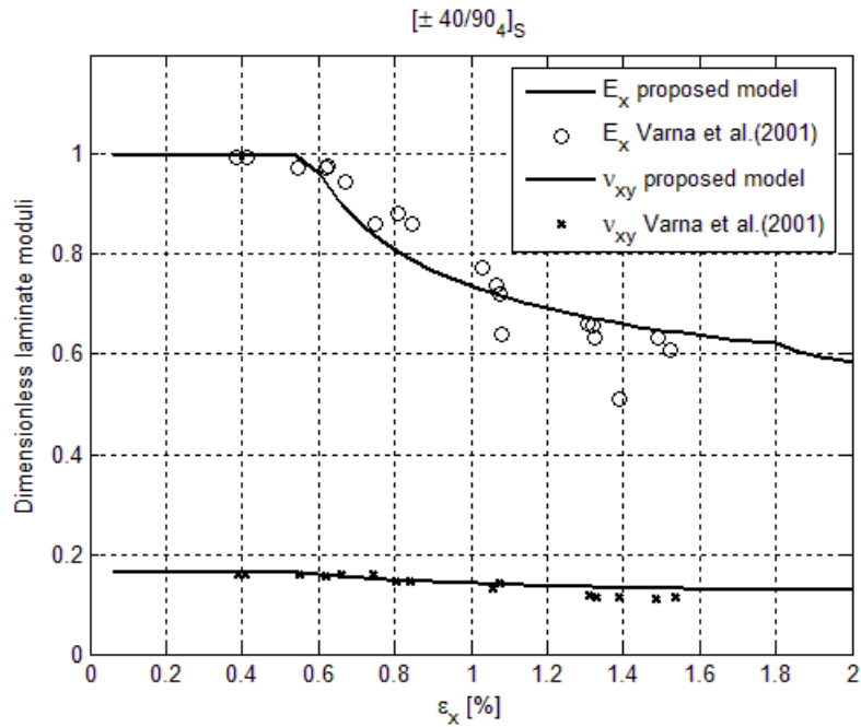
Figure 10. Loss of laminate modulus modulus E_x / \bar{E}_x and \nu_{xy} as a function of applied strain for a [40/-40/90 4 ] S laminate.
